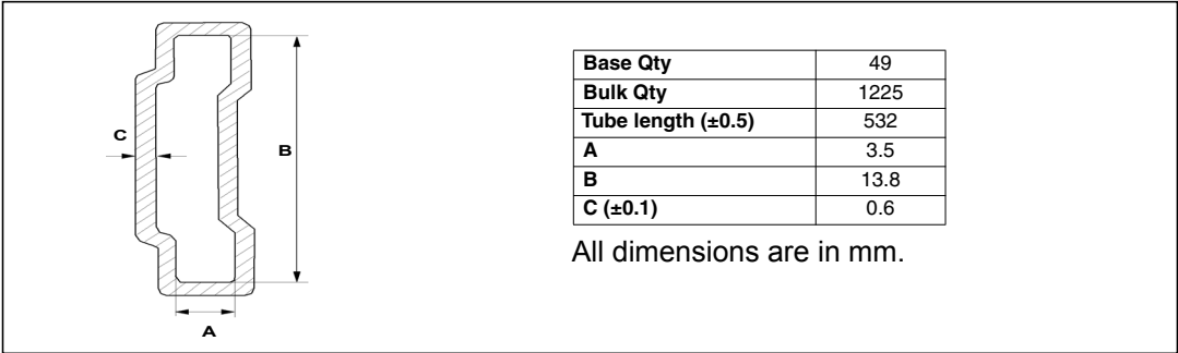
Figure 28. PowerSSO-36 TP tube shipment (no suffix)
