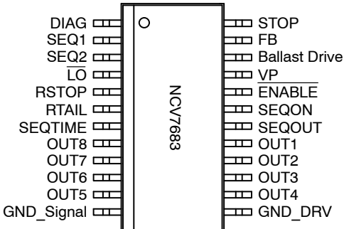
Figure 2. Pinout Diagram
