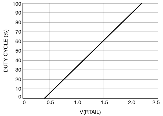
Figure 14. Duty Cycle vs. V(R_{TAIL})
