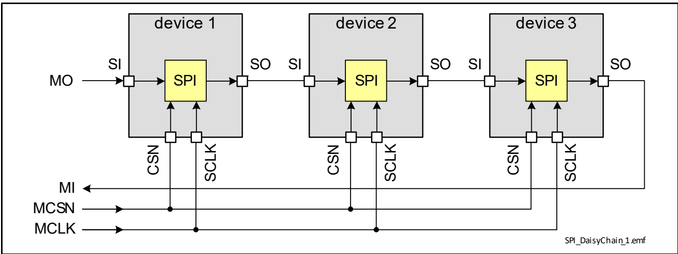
Figure 37 Daisy Chain Configuration
