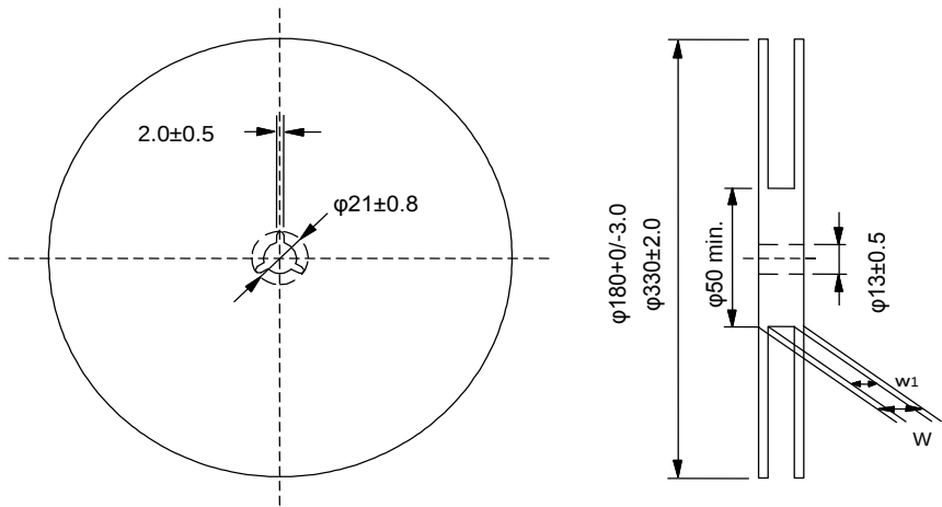
Fig.3 Taping Diagram
