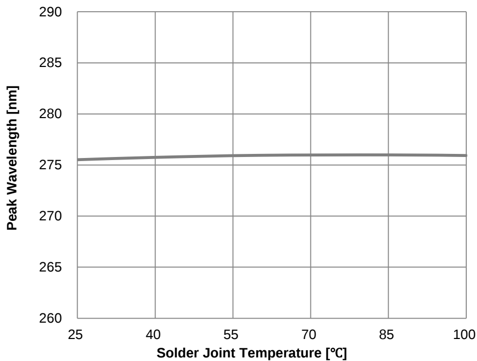
Fig 6. Solder Joint Temperature vs. Peak Wavelength, I_F=30\text{mA}
