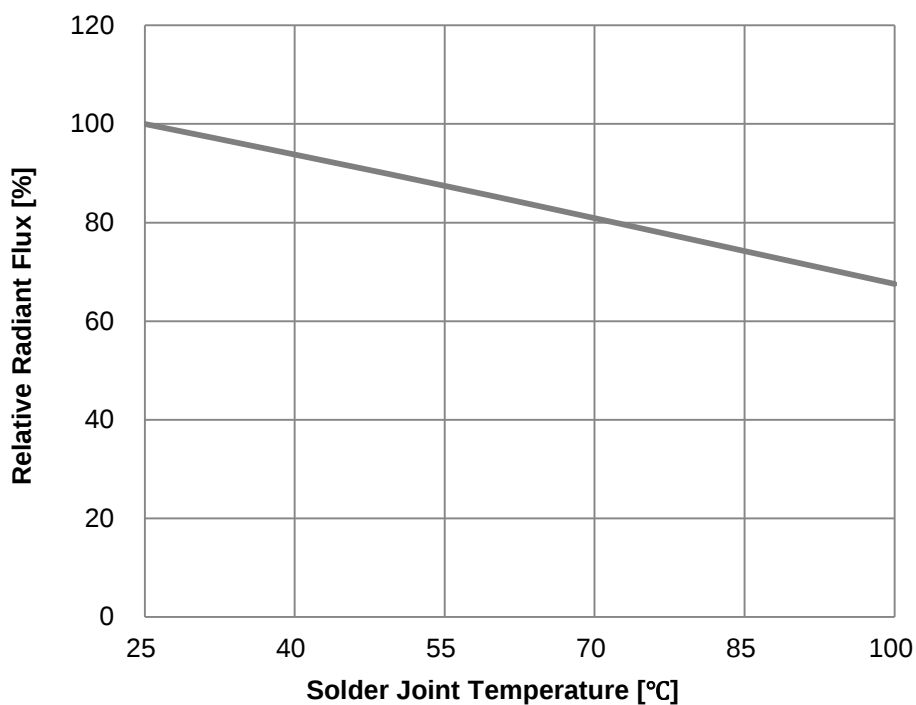
Fig 5. Solder Joint Temperature vs. Relative Radiant Flux, I_F=30\text{mA}
