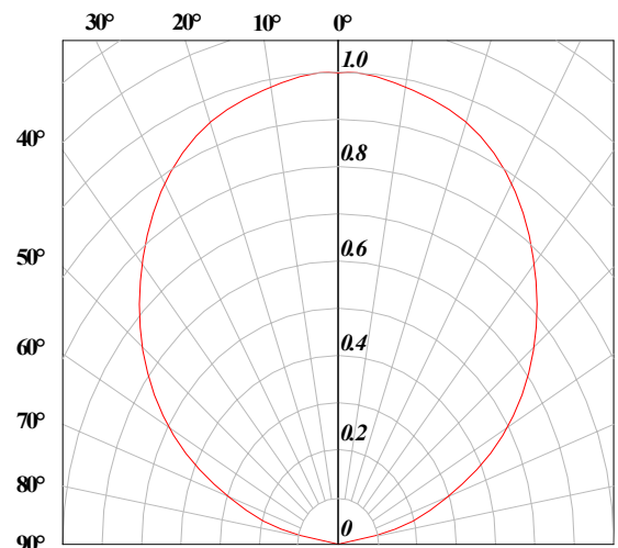
Radiation Pattern
